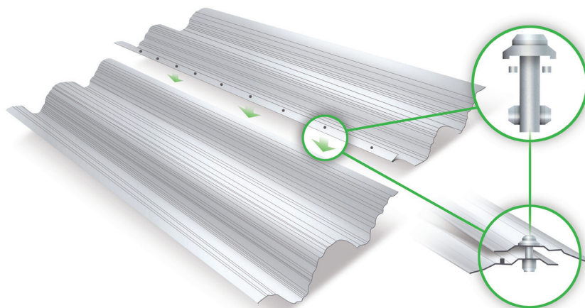
PANEL DETAILS
